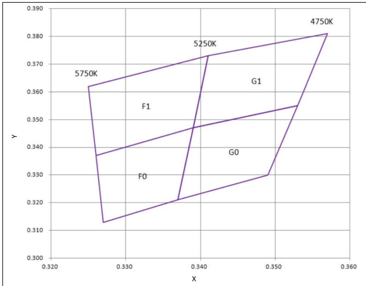
Chromaticity Coordinates Classifications ( I_F = 20\text{mA} ):
