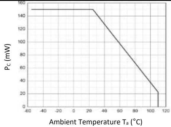
Collector Power Dissipation v.s. Ambient Temper.
