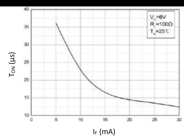
Turn On Time v.s. Forward Current
