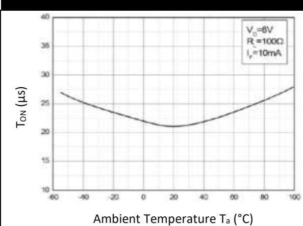
Turn On Time v.s. Ambient Temperature
