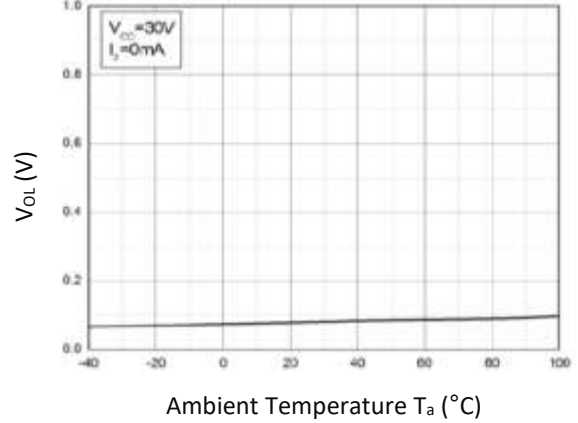
Low Level Output Voltage v.s. Ambient Temperature
