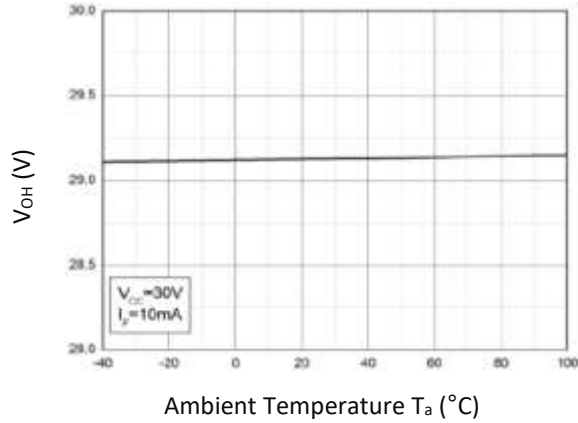
High Level Output Voltage v.s. Ambient Temperature
