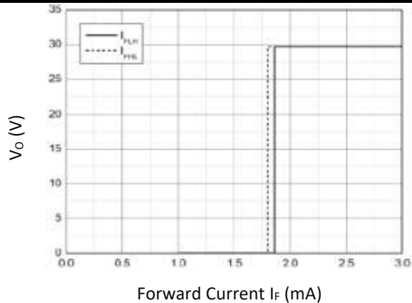
Output Voltage v.s. Forward Current
