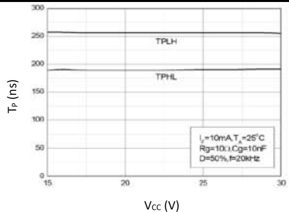
Propagation Delay v.s. Supply Voltage
