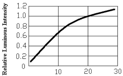
Luminous Intensity vs. Forward current Ta=25°C
