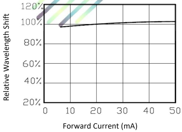
Wavelength v.s. Forward Current
