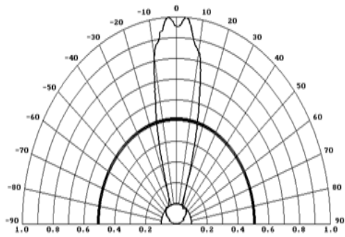
Directive Radiation
