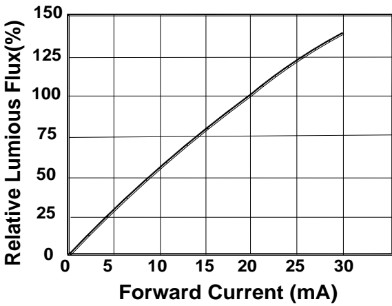
5). Electrical Characteristics
