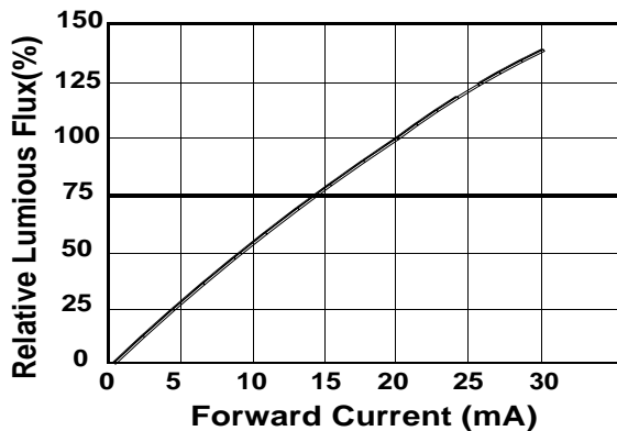
5).Electrical Characteristics
