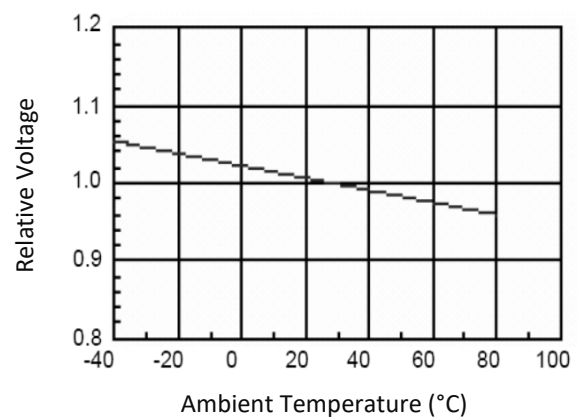
Relative Voltage v.s. Ambient Temp.
