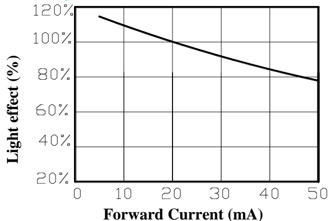
8). Light effect VS Current
