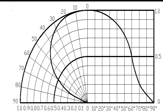
Directive Radiation
