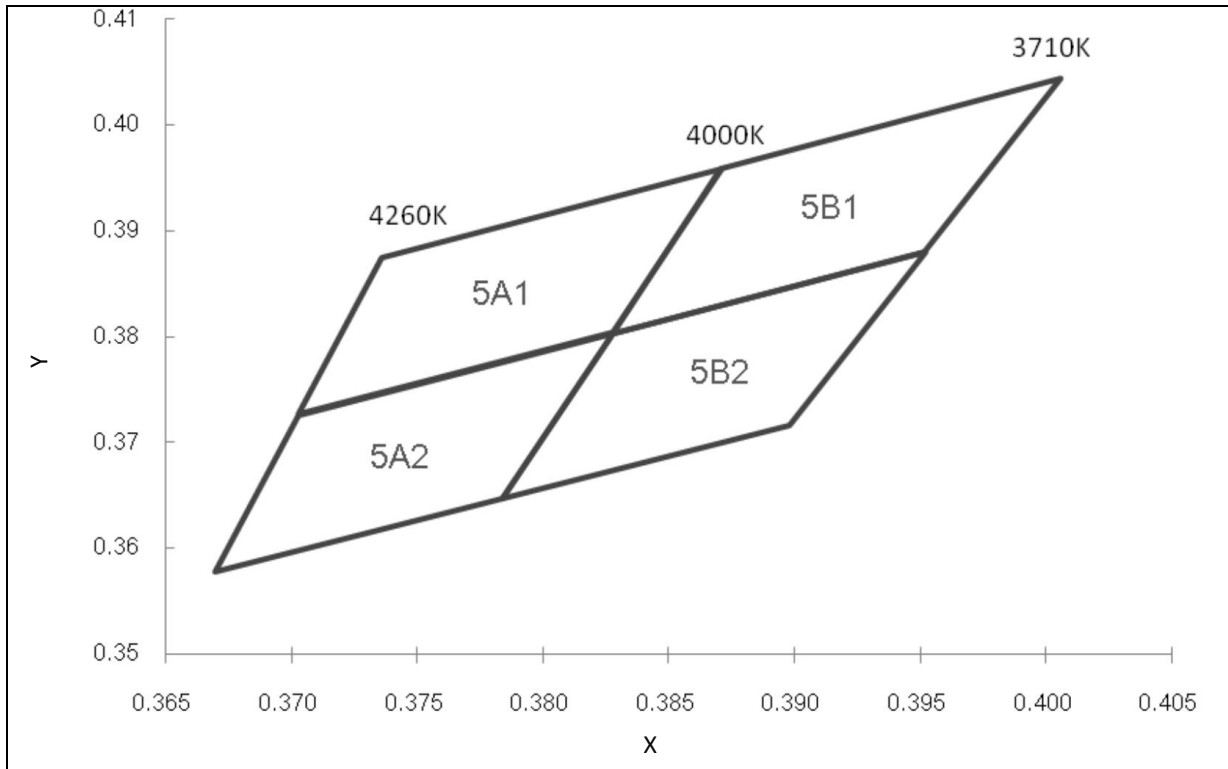
Chromaticity Coordinates Classifications ( I_F = 60\text{mA} ):
