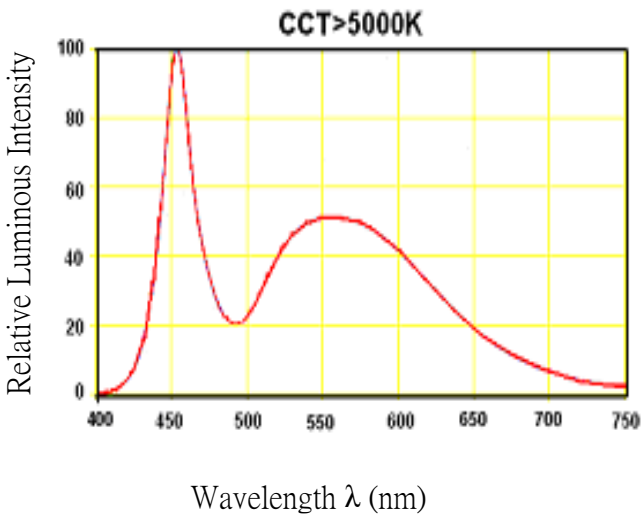
Fig.3 Wavelength Characteristics (Ta=25°C)
