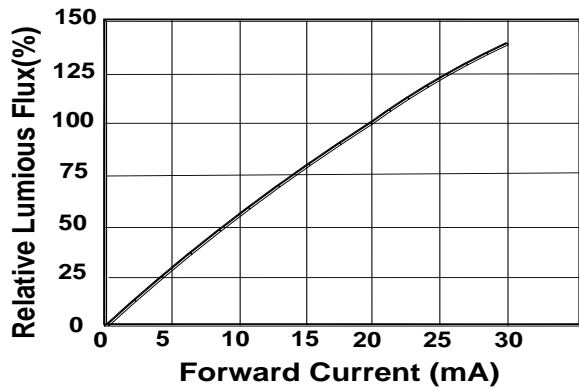
5). Electrical Characteristics
