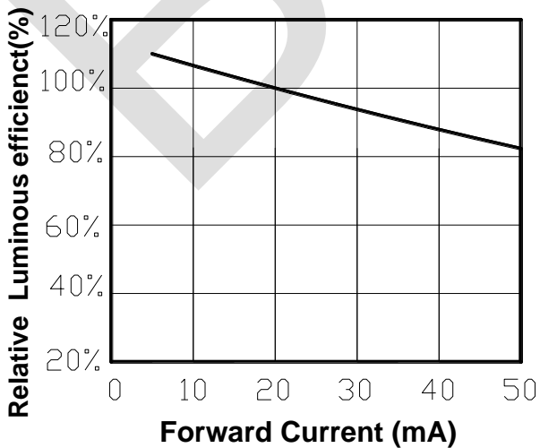
7). Relative Emission Efficiency. Current
