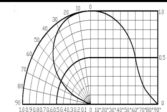
Directive Radiation
