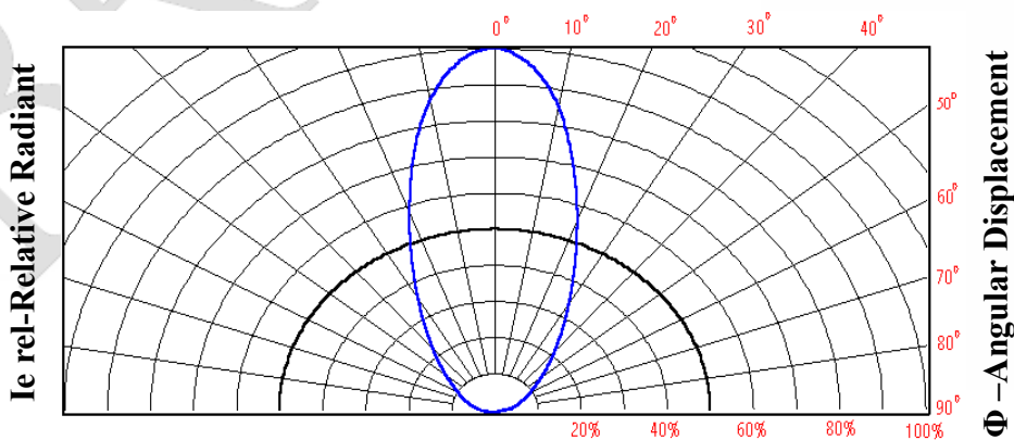
Relative Radiant Intensity vs .Angular Displacement
