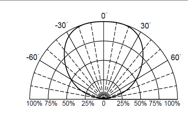
Directive Radiation
