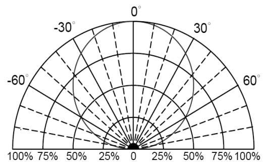
Directive Radiation
