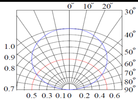
Directive Radiation
