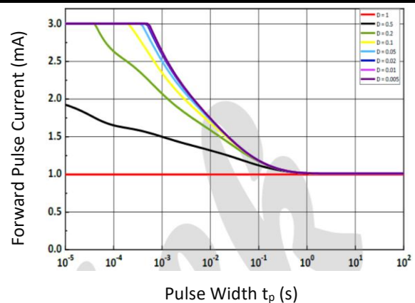
Permissible Pulse Handling Capability I_F = f(t_p) ; D =Duty Cycle; T_s=85^\circ\text{C}
