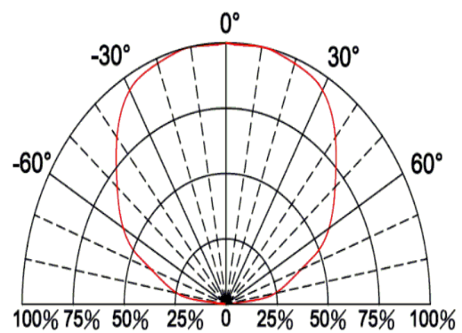
Directive Radiation
