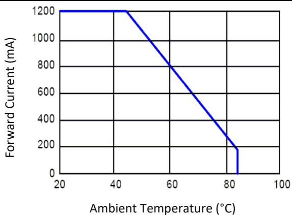
Max. Driving Current v.s. Ambient Temperature
