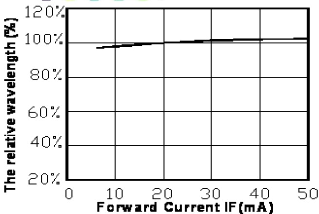
7). Wavelength and current
