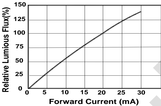
5).Electrical Characteristics
