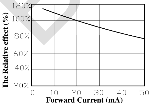
7). Relative Emission Efficiency. Current
