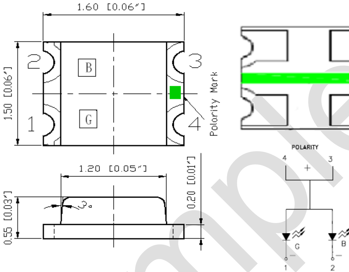
RECOMMEND PAD LAYOUT
