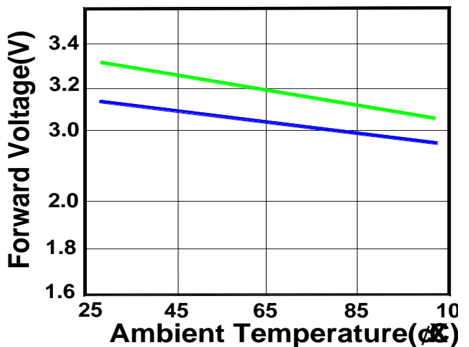
6). Forward Voltage Vs Temperature
