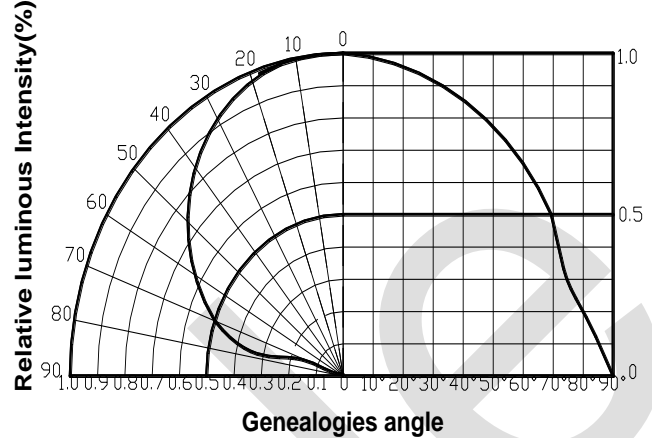
2). Typical Spatial Distribution
