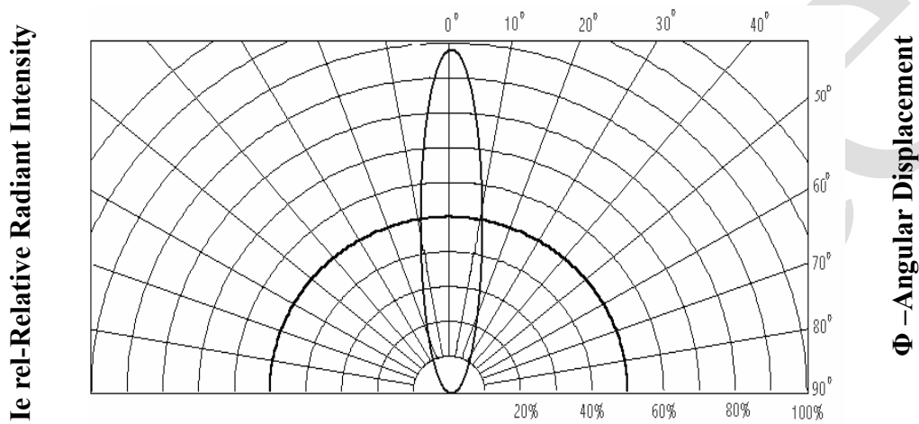
Relative Radiant Intensity vs .Angular Displacement
