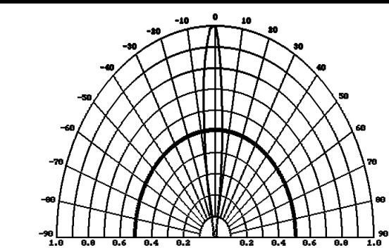
Directive Radiation
