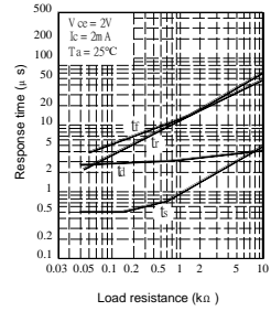
Response time Vs. Load resistance
