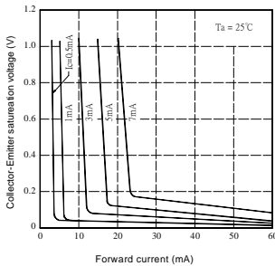
Collector-Emitter saturation voltage Vs. Forward current
