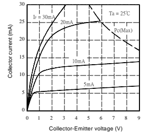
Collector current Vs. Collector-Emitter voltage
