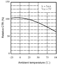
Relative CTR Vs. Ambient temperature
