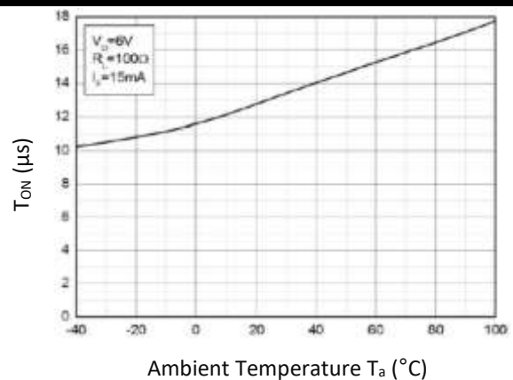
Turn On Time v.s. Ambient Temperature
