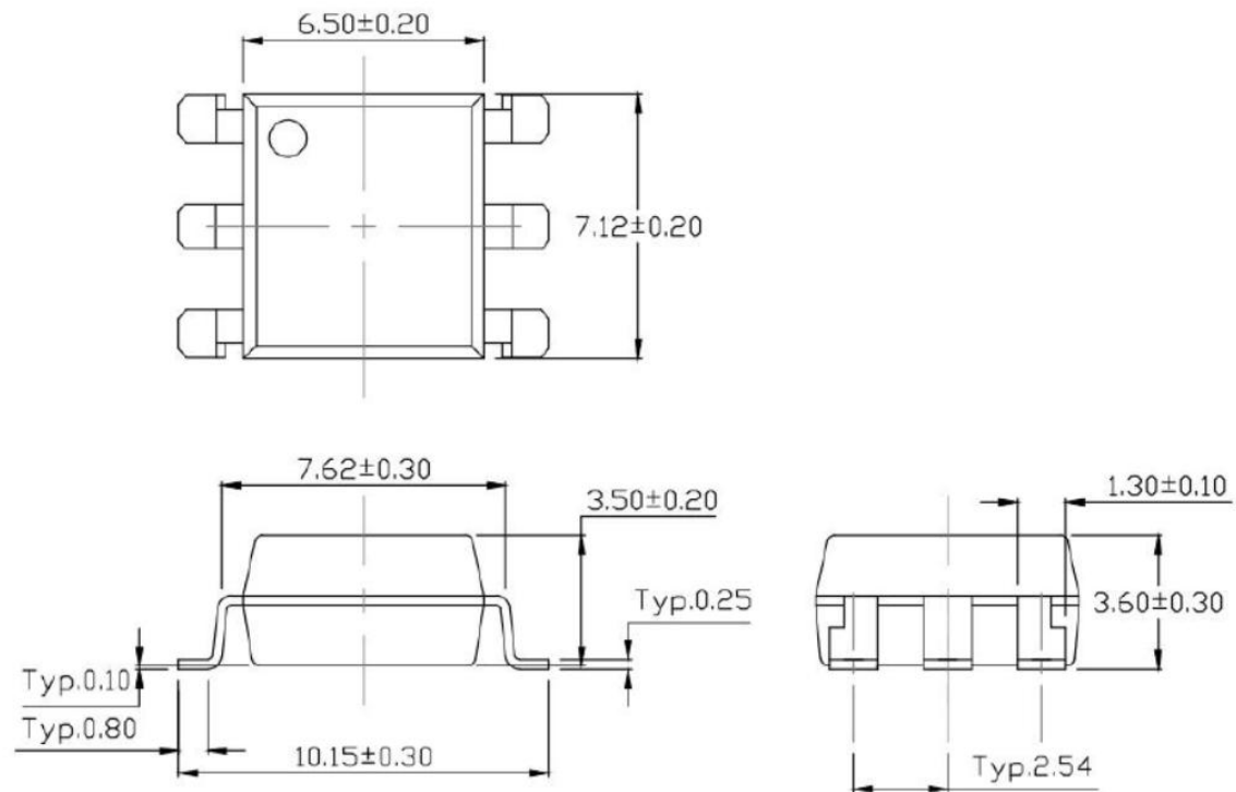
Surface Mount Low Profile Lead Forming - SMD (SL Type)
