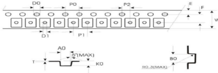
Tape Dimension
