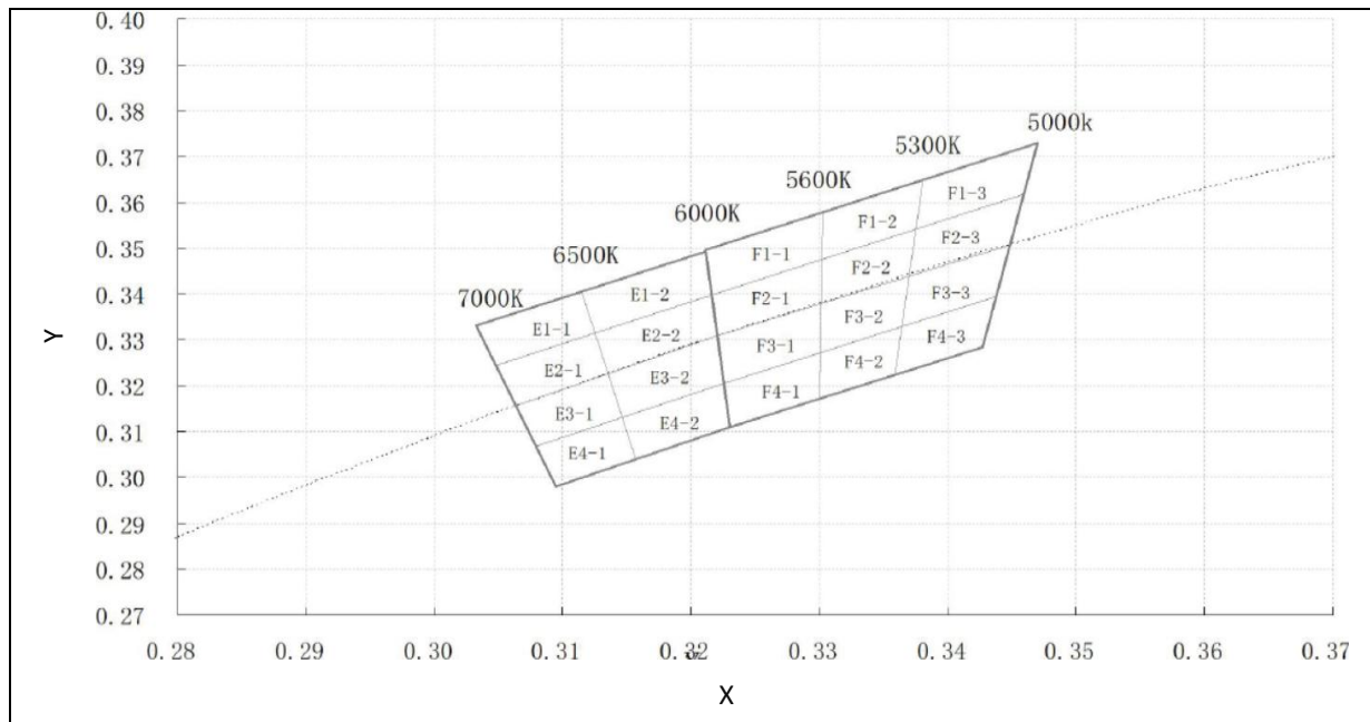
Chromaticity Coordinates Classifications ( I_F = 20\text{mA} ):
