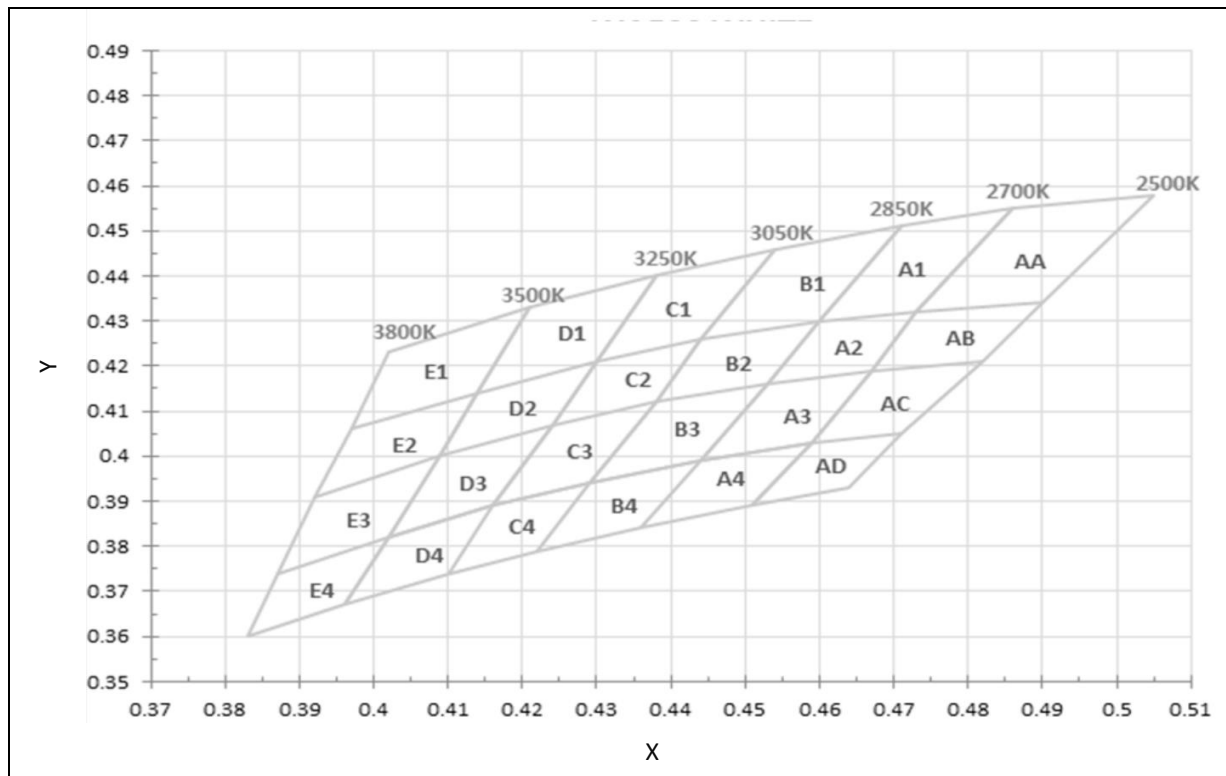
Chromaticity Coordinates Classifications ( I_F = 700\text{mA} ):
