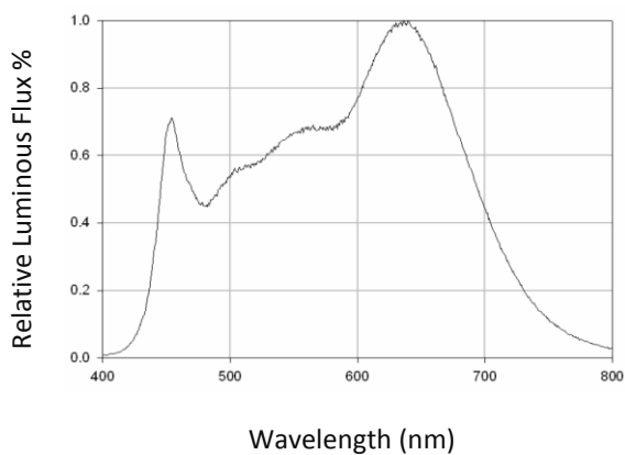
Luminous Spectrum
