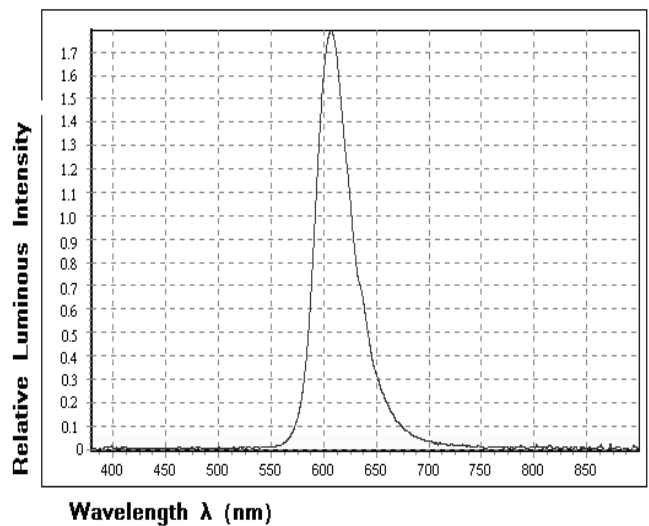
6). Wavelength Characteristics ( T_a=25^{\circ}C )
