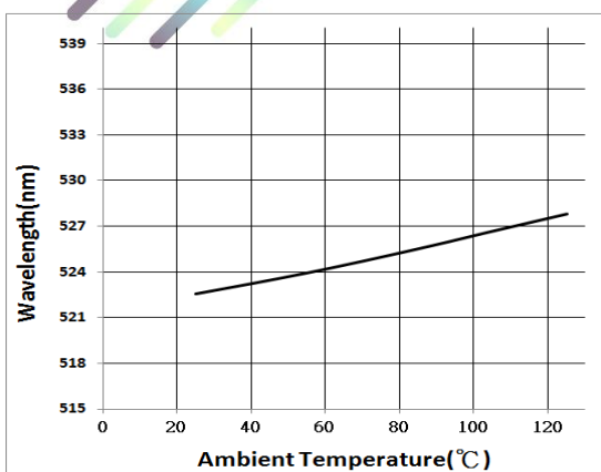
7). Relative Wavelength & Temperature
