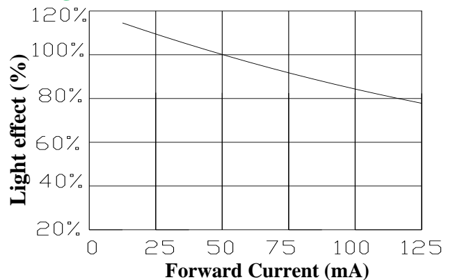
8). Light effect VS Current
